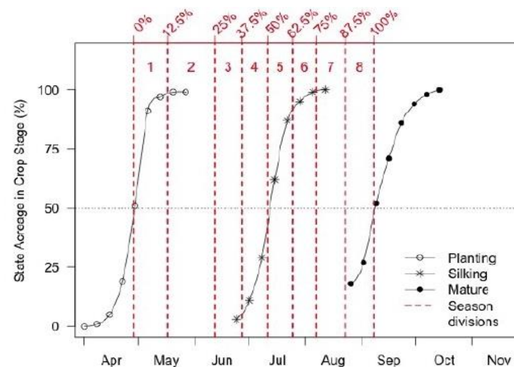
Figure 2. Simulation of crop choice (upper panel) and timing of crop development (right panel).
