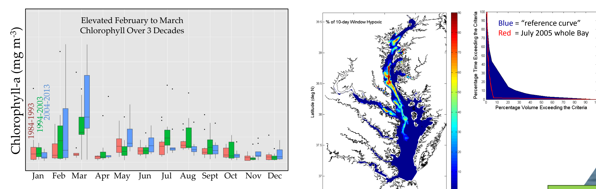
Figure 4. Seasonal cycles of chlorophyll-a over each of the past three decades show changes in intra-annual variability (upper left panel). Simulated oxygen distribution in July and associated cumulative frequency diagram to assess criteria (upper right panel).
